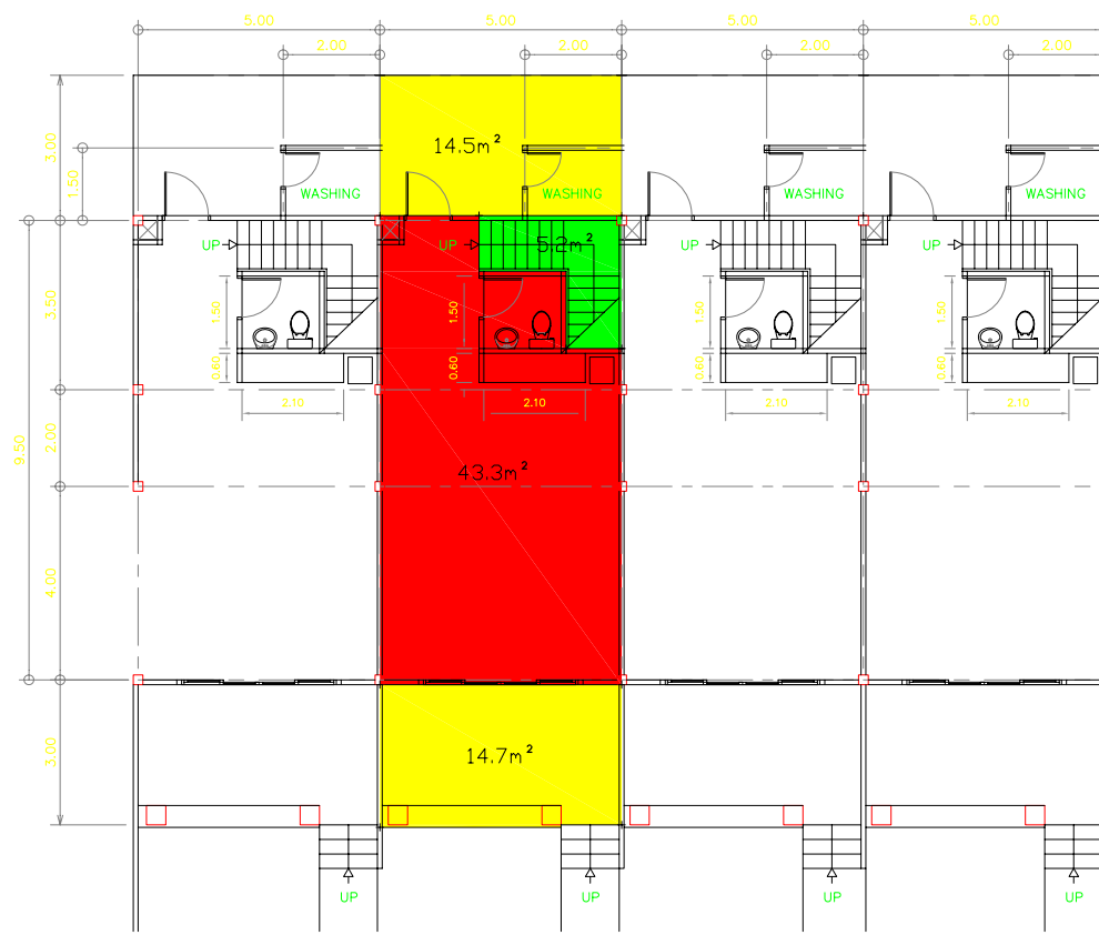
Type A 1st FLOOR PLAN
